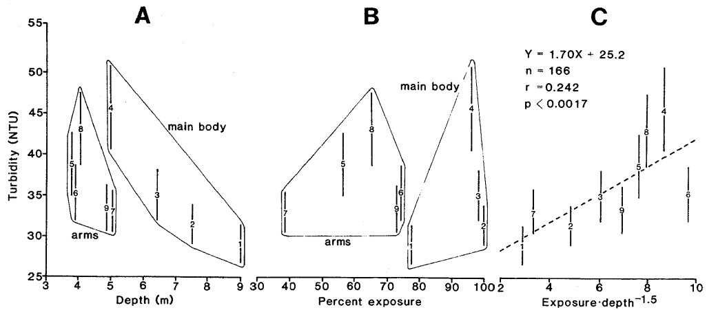
Figure 5. Relationship between turbidity and a) depth, b) percent exposure, and c) exposure \cdot depth -1.5 . The numbers indicate stations. Error bars indicate \pm 1 standard error. Depth was the average depth in a 750-m-radius circle drawn around each station. Percent exposure was the percent area in a 500-m-radius circle around each station that was water.
