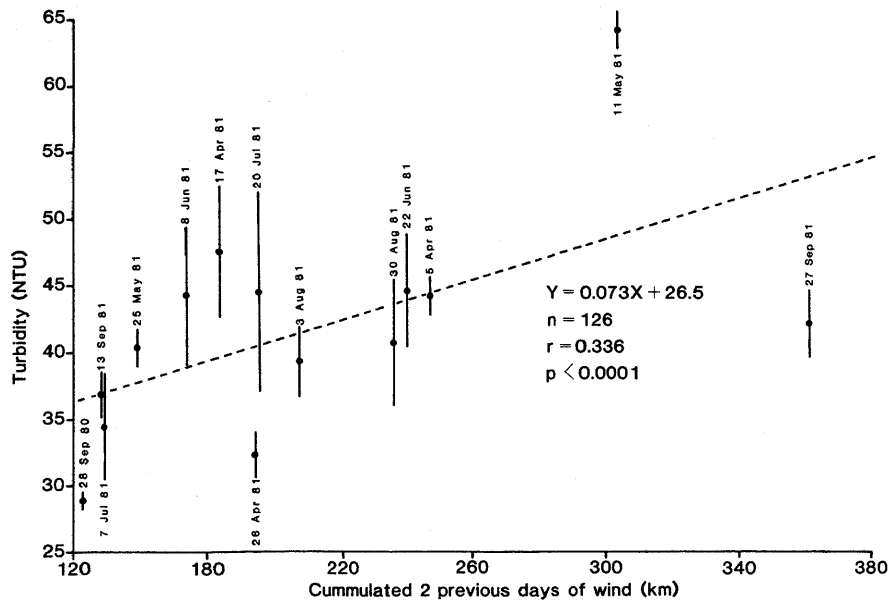
Figure 4. Relationship between turbidity and amount of wind. Only those dates for which all nine stations were sampled are shown. Points are the mean of the nine stations for the indicated date. Error bars indicate \pm 1 standard error.
