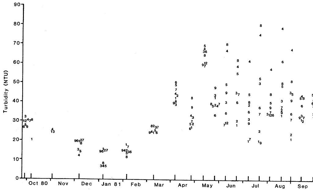
Figure 3. Temporal and horizontal changes in turbidity. The numbers correspond to stations.
