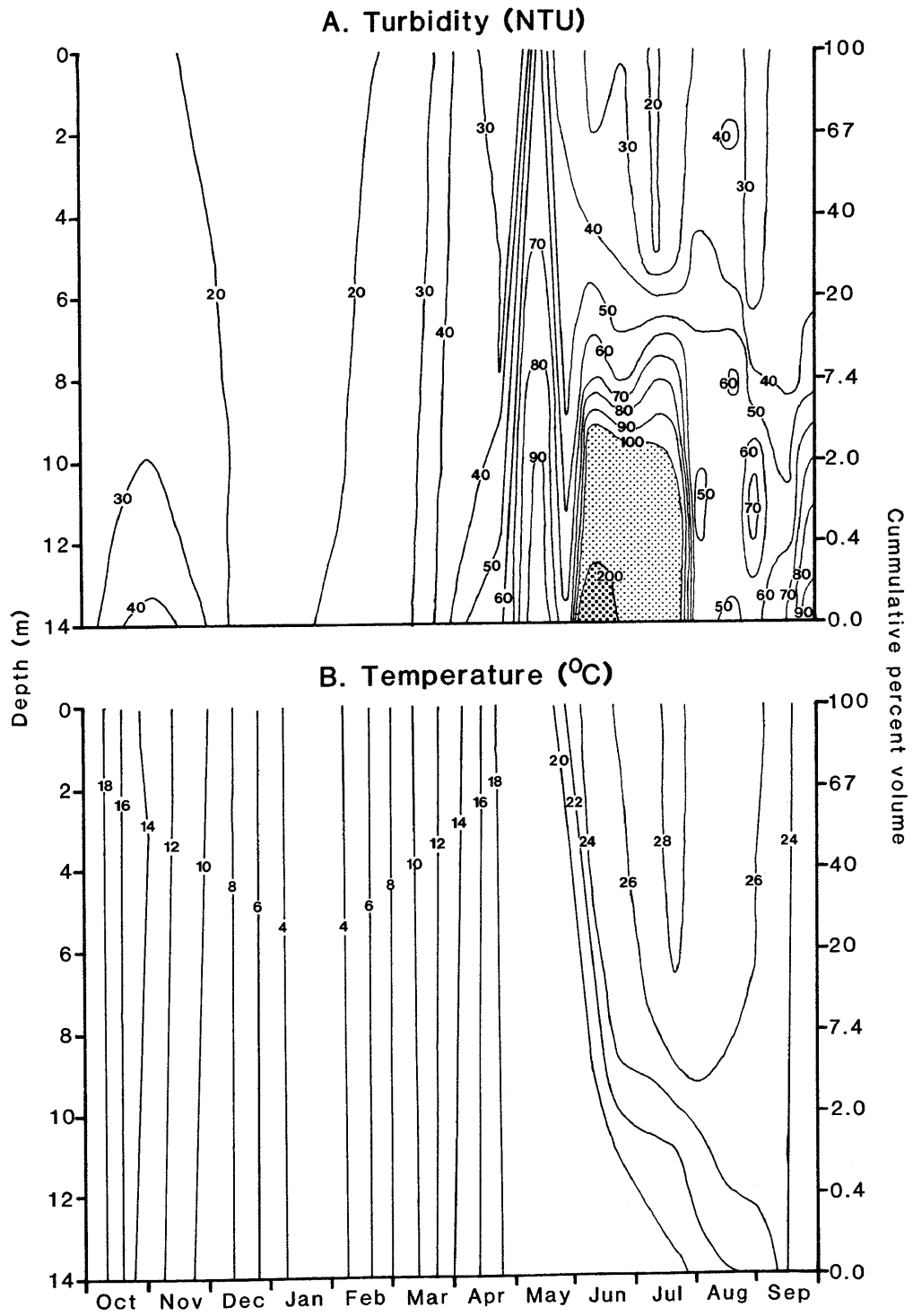
Figure 2. Temporal and vertical distributions of a) turbidity and b) temperature at Station 1.
